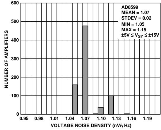
Figure 43. Voltage Noise Density at 1 kHz
