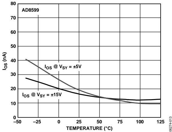
Figure 16. Input Offset Current vs. Temperature
