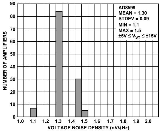
Figure 40. Voltage Noise Density at 10 Hz
