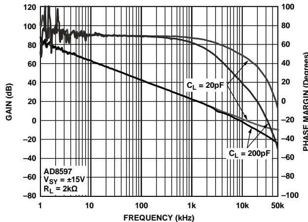
Figure 33. Gain and Phase vs. Frequency
