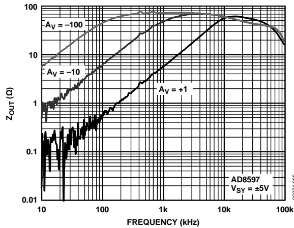
Figure 35. Closed-Loop Output Impedance vs. Frequency
